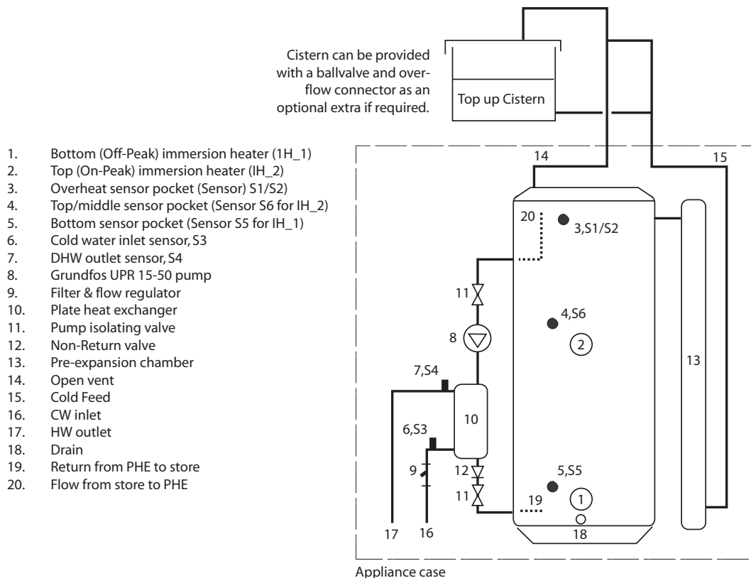
Schematic Hydraulic Arrangement
