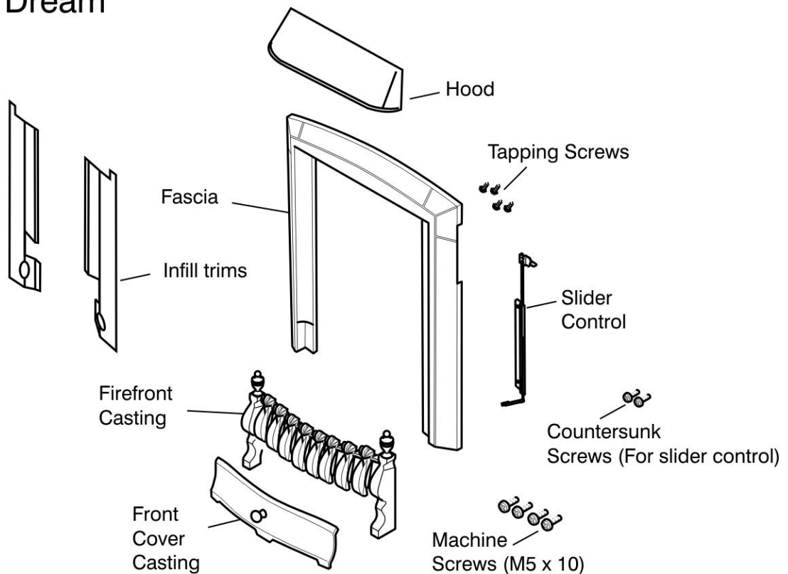
Figure 6. Pack contents continued
