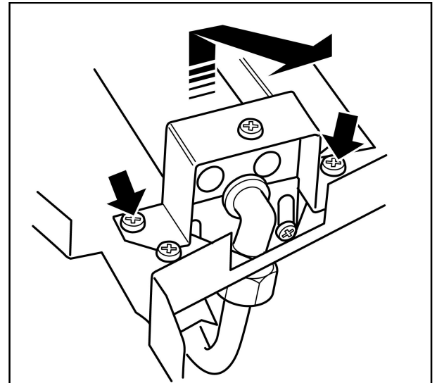
Figure 41. Removal of burner
